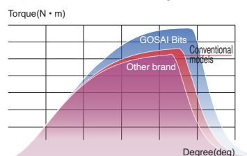
Comparison test with twisting tester
