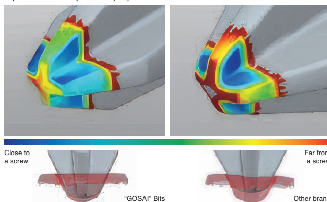
Tip-end 3D comparison (+0)
